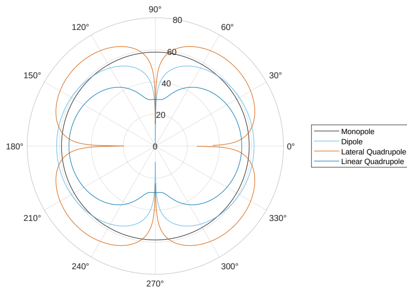
Figure 2: Source directivity patterns for a monopole, dipole, lateral quadrupole, and a linear quadrupole.
