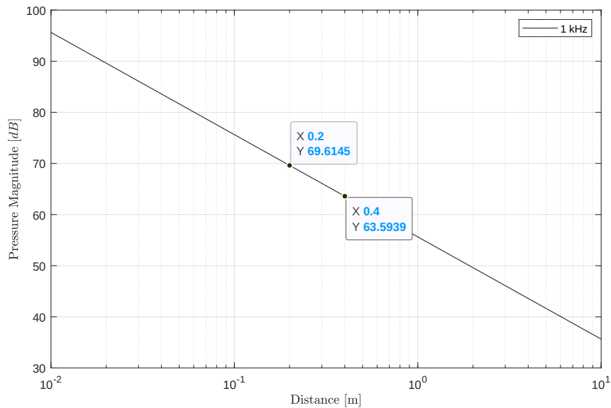
Figure 1: Monopole spherical spreading sound pressure level for a 1 kHz.
