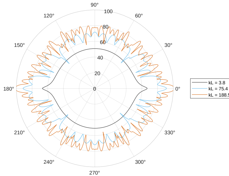
Figure 4: Line source directivity patterns for frequencies of 100 Hz, 2 kHz, and 5 kHz with large source separation.
